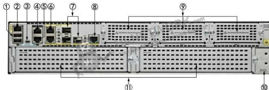
Figure 3 shows the back panel of Cisco ISR4351/K9.
