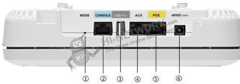
Figure 2 shows AIR-AP1852E Ports and Connections.
