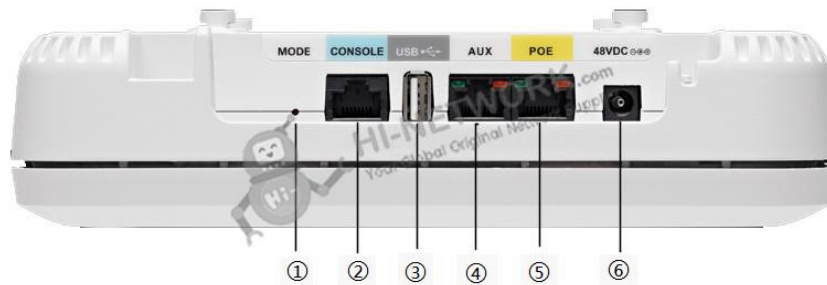
Figure 3 shows AIR-AP1852I Ports and Connections.
