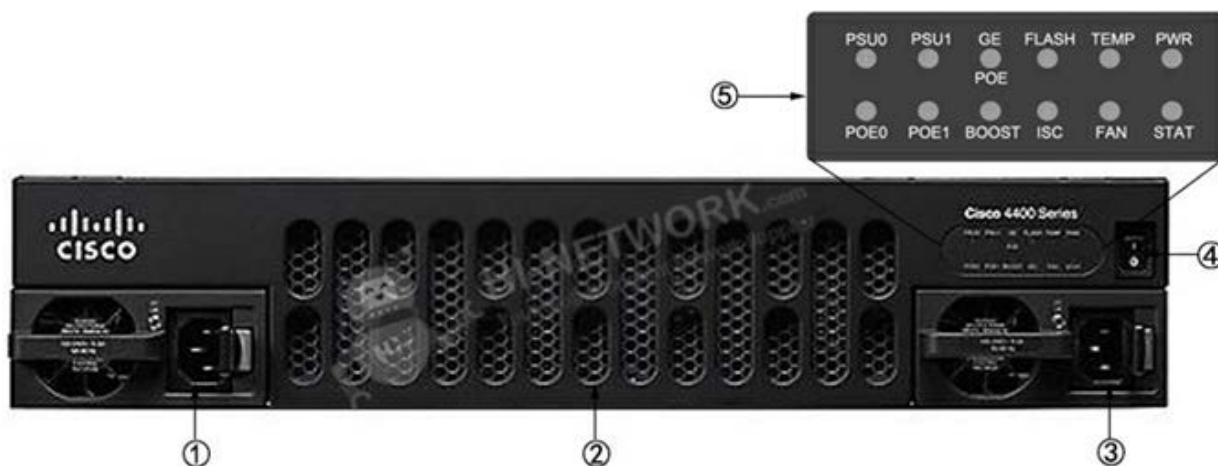
Figure 2 shows the front panel of Cisco ISR4451-X-VSEC/K9.
